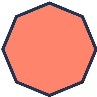
octagon
