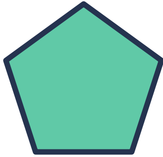
pentagon
